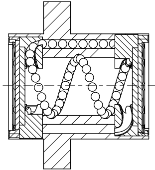
Fig 1.6.4 Y, YA, H, A, J - type nut
